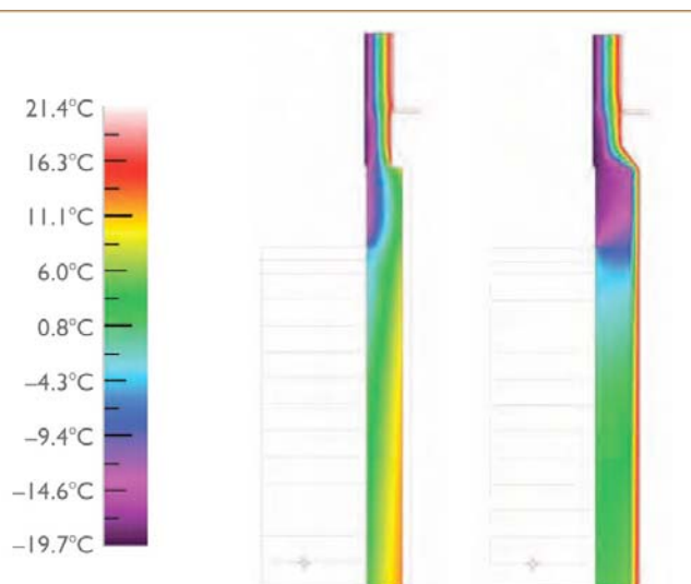
Figure 3 (left): Infrared THERM Simulation of an Uninsulated Basement Wall —Insulation or no insulation, the thermal gradient is away from the foundation wall.
